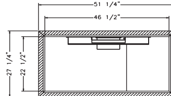
FROSTER-B-50-US
